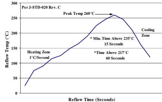
Figure 50. Recommended linear reflow profile using Sn/Ag/Cu solder.
